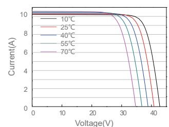
Current-Voltage Curve JAM60S10-330/PR
